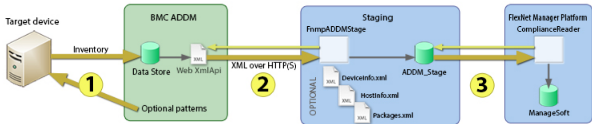
Figure 1: Process overview
