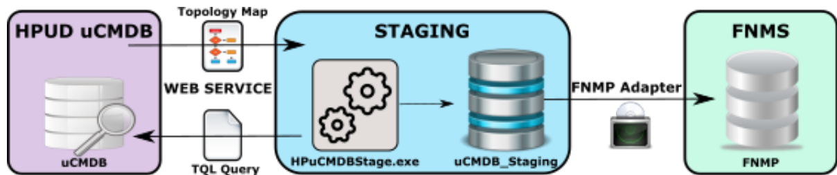
Figure 5: Architecture and working of the HPE-UD adapter
